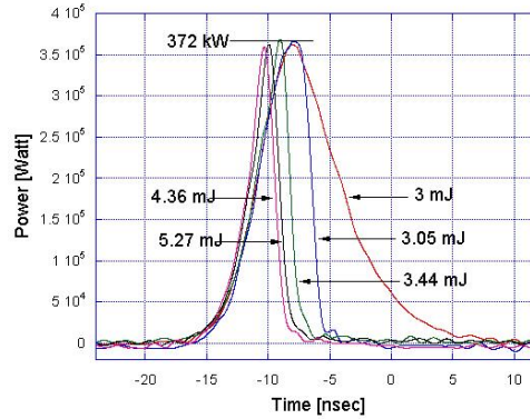
Figure 11: Transmitted waveforms below and above optical breakdown threshold, w_0 = 7.45 mm, t_0 (FWHM) = 7.5 ns.
