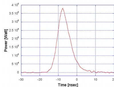
Figure 2 Temporal shape of the laser pulse. The pulse width is 7.5 ns FWHM.
