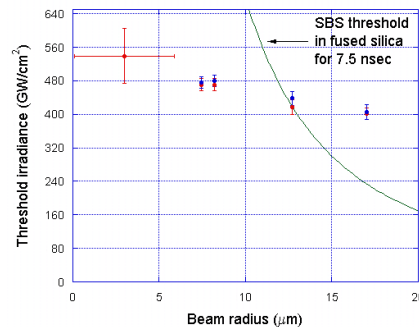
Figure 14: Damage threshold irradiances at different beam radii, the left most and the lower data points for linearly polarized light, and the upper data points for circularly polarized light.
