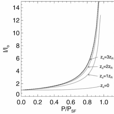
Figure 7: Irradiance enhancement for different depths of focus.
