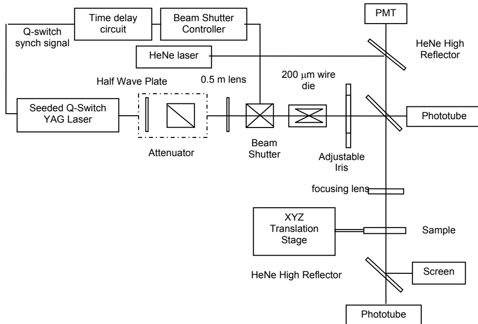
Figure 1: Experimental set-up.
